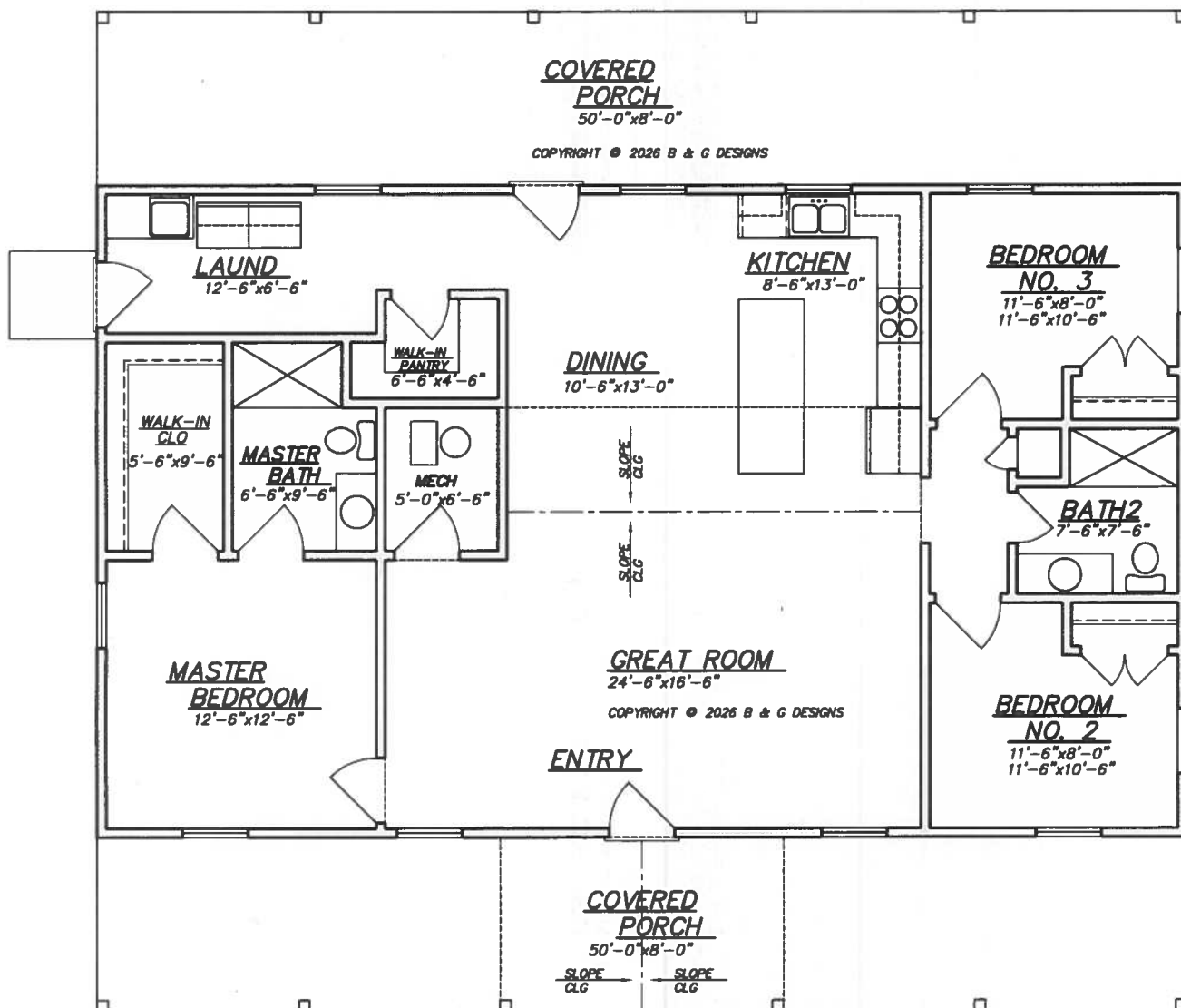
FLOOR PLAN 50'-0" x 46'-0"
